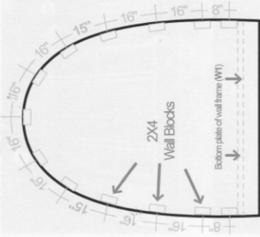
Figure 6. 2X4 wall blocks: spacing measurements
